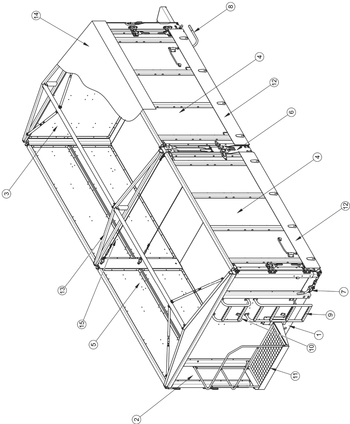
FIGURE 3.2 Benne
