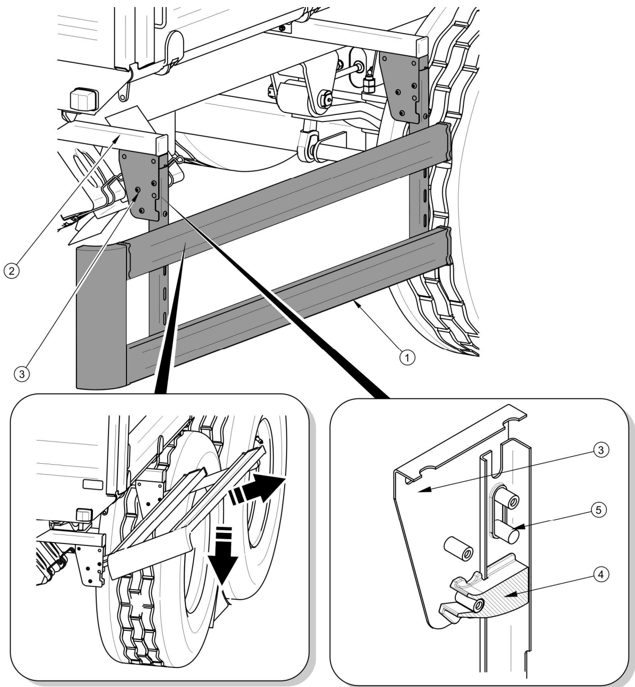
FIGURE 4.8 Barre anti-encastrement gauche
