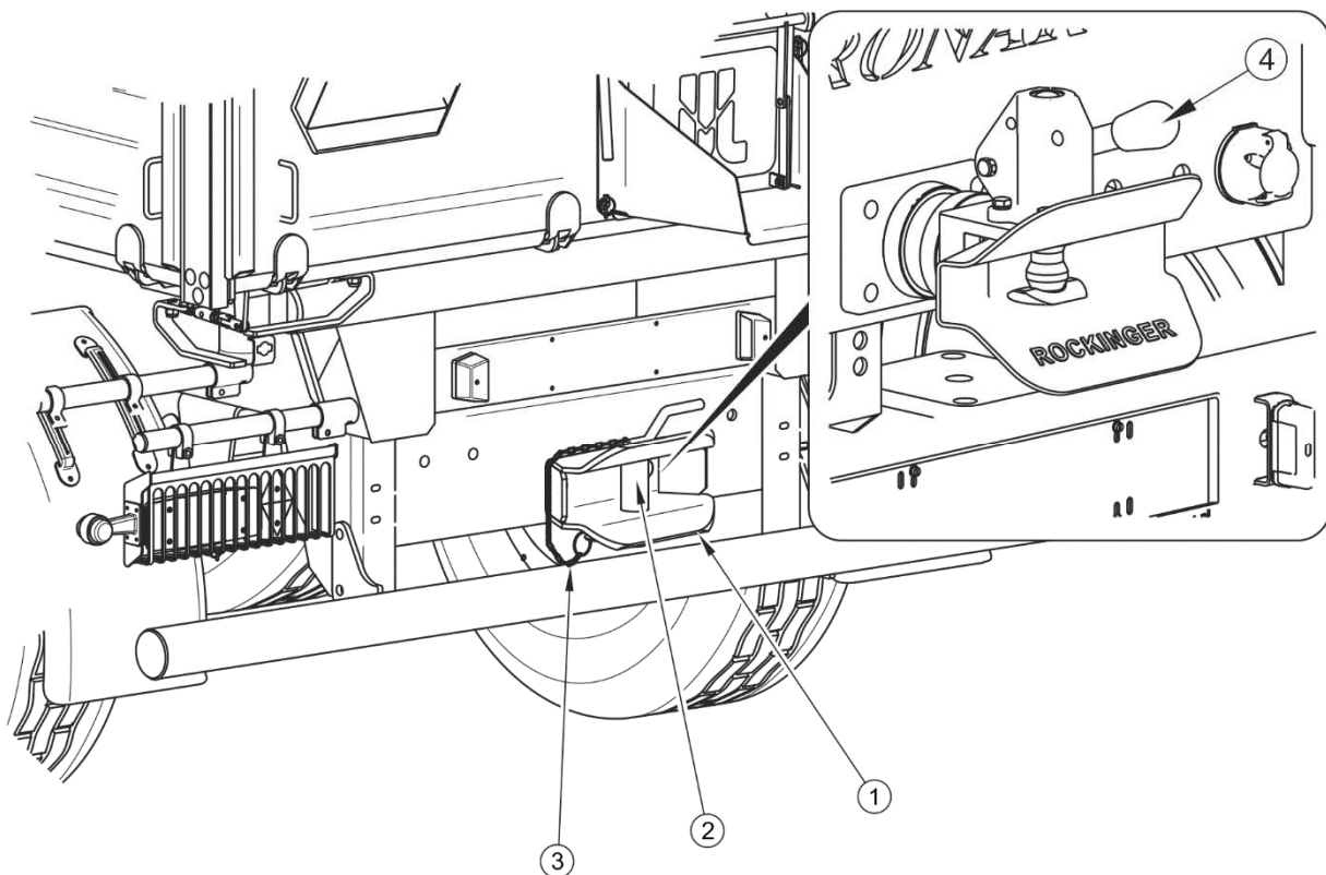
FIGURE 4.2 Attelage arrière
