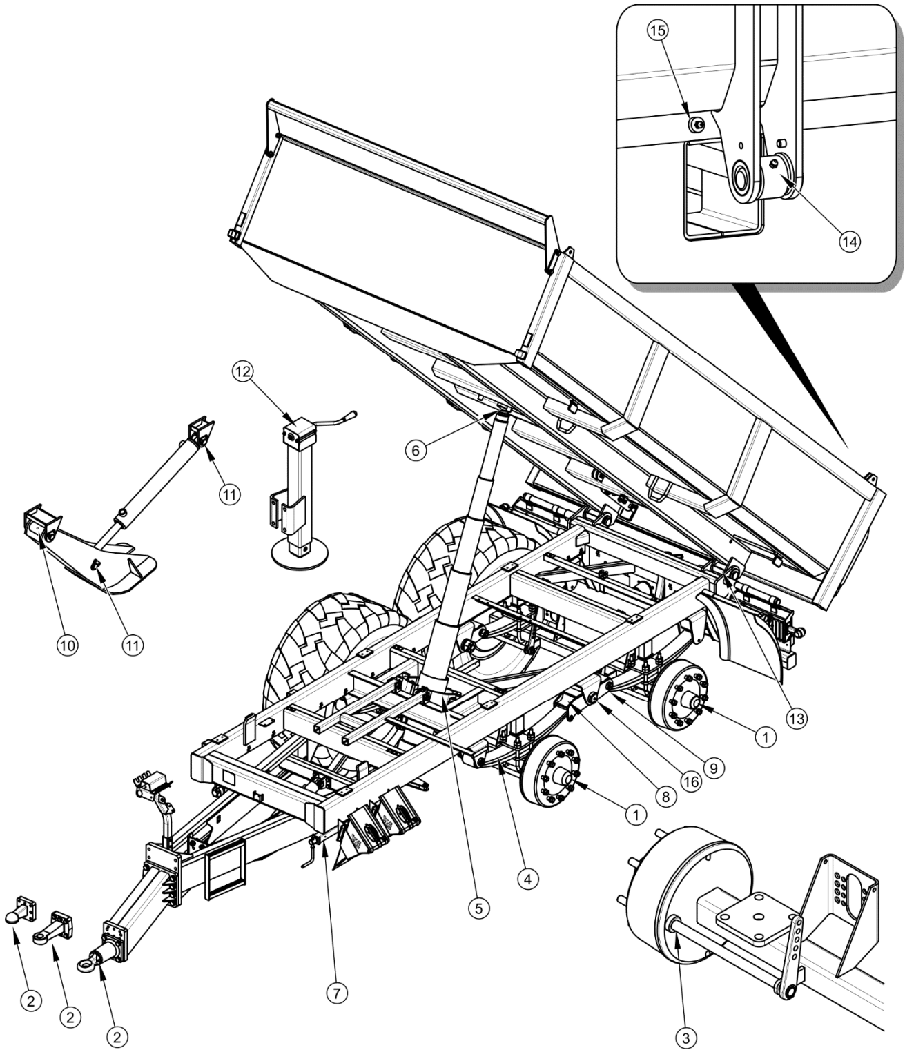
FIGURE 5.11 Points de lubrification de la remorque
